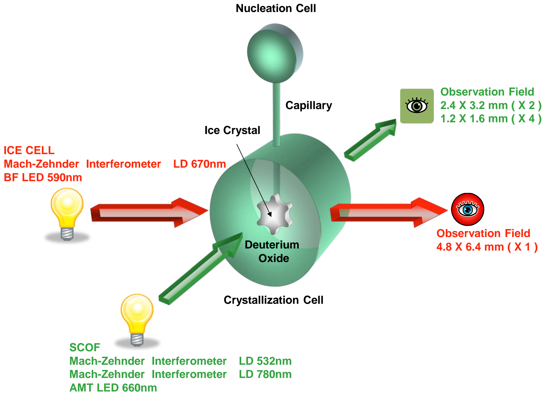
Optical Path of ICE-CELL Observation
